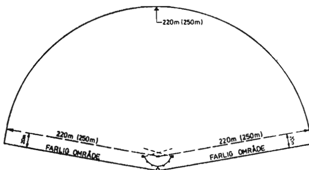
Figur 21 Lerduebane – skeet
